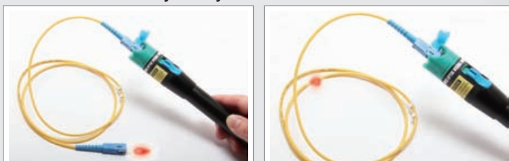
Continuity test
