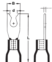
Locking Spade Terminals (Vinyl)
